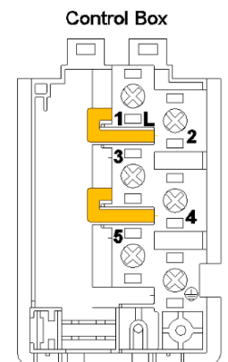
Heater de-rated to 2kW
