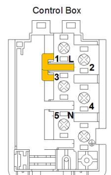
Heater de-rated to 4kW
